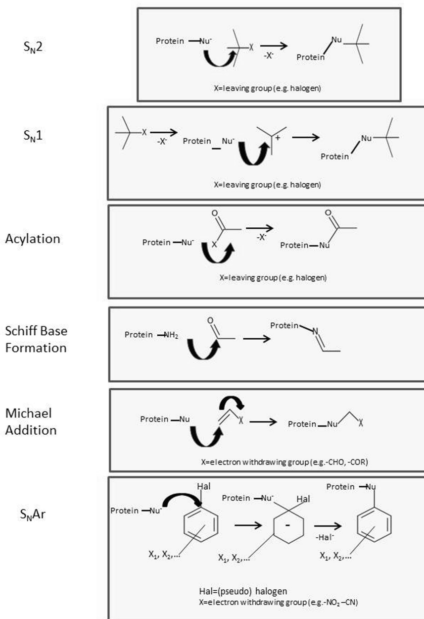
Figure 3 Mechanisms of covalent binding to cellular nucleophiles (DNA, proteins) *Nu- nucleophilic site of molecule
