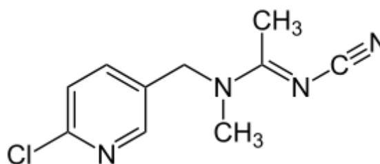
Figure 1 Chemical structure of acetamiprid
