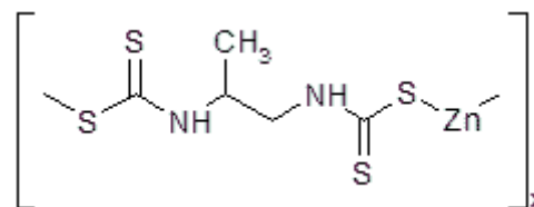
Figure 2 Chemical structure of propineb
